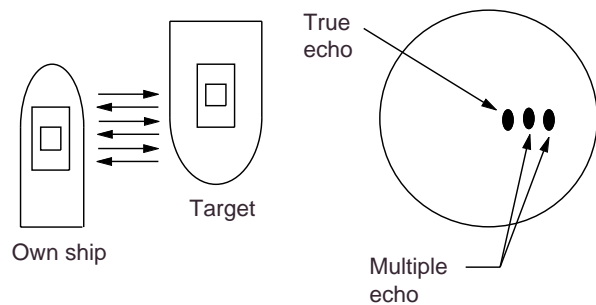
Figure 2-2 Multiple echoes
